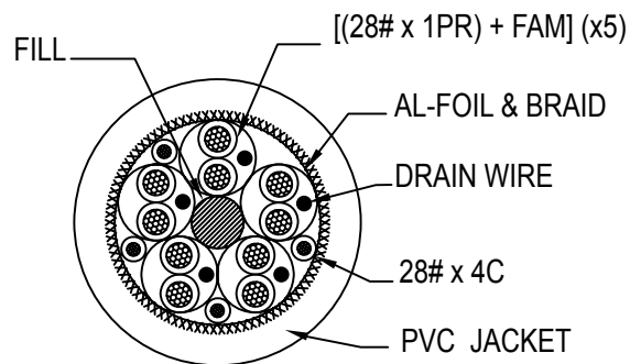
SECTION: A-A FAM = FREE-EDGE AL-FOIL MYLAR
