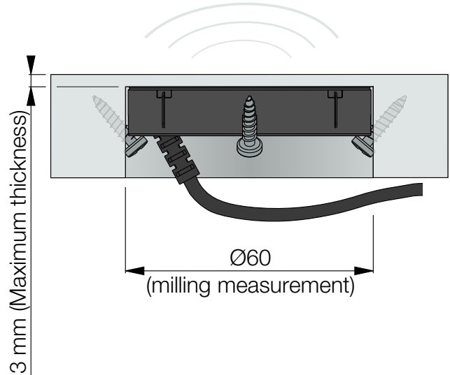
Side View (Integrated into table)
