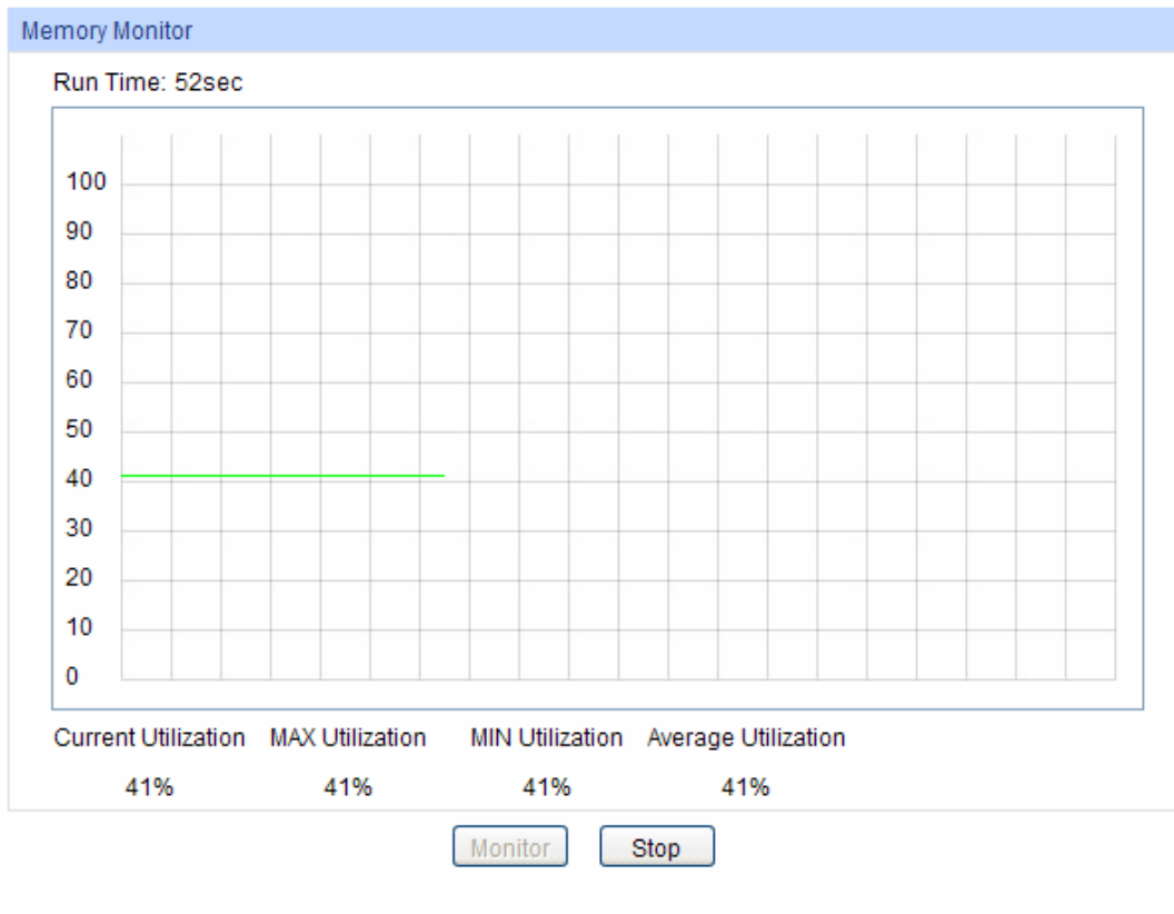
Figure 15-2 Memory Monitor
