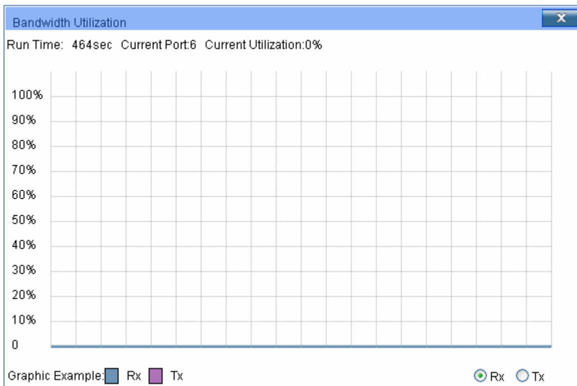
Figure 4-3 Bandwidth Utilization
