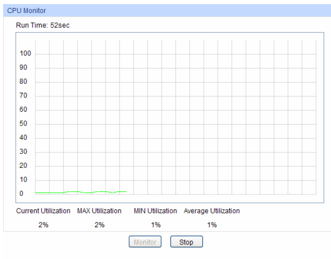
Figure 15-1 CPU Monitor
