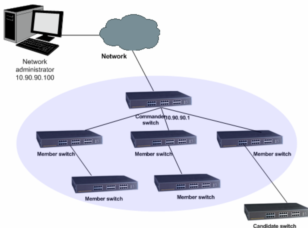
Figure 14-1 Cluster topology
