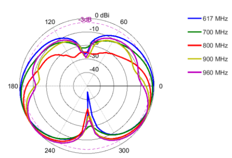
Elevation: 617 - 960 MHz
