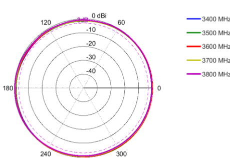
Azimuth: 3400 - 3800 MHz
