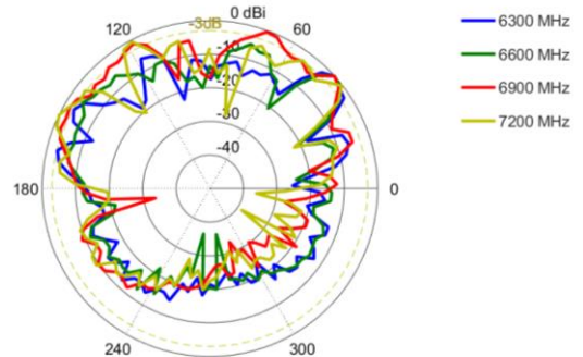
Elevation: 6300 – 7200 MHz
