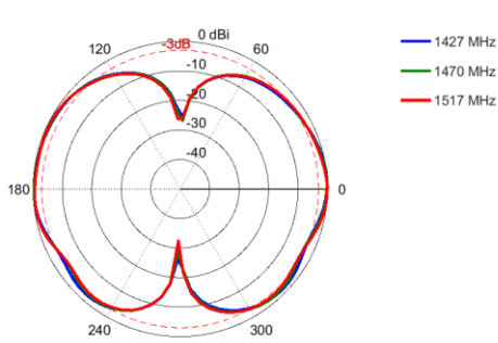
Elevation: 1427 - 1517 MHz
