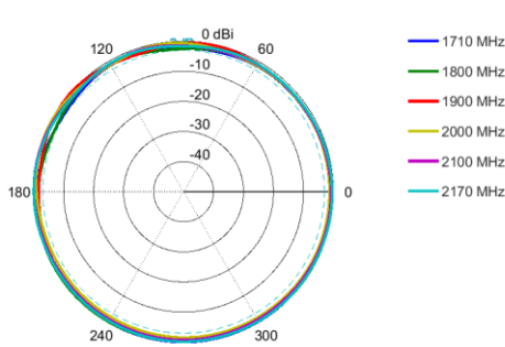
Azimuth: 1710 - 2170 MHz
