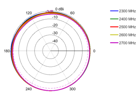
Azimuth: 2300 - 2700 MHz
