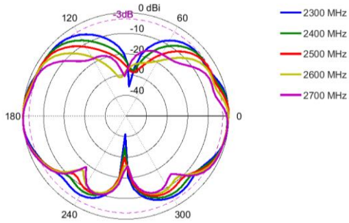
Elevation: 2300 – 2700 MHz
