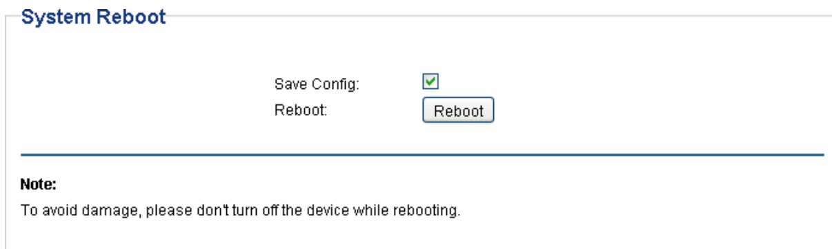
Figure 4-12 System Reboot
