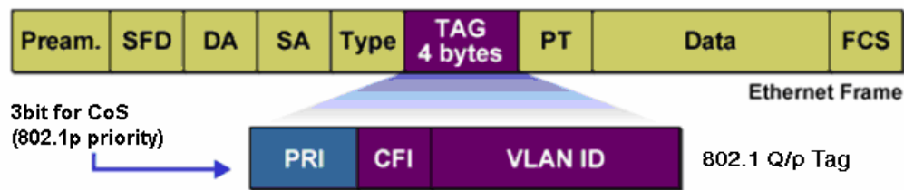
Figure 6-2 802.1Q frame
