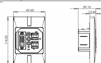
Jack PC with US Frame
