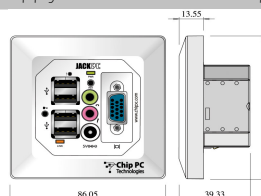
Jack PC with EU Frame
