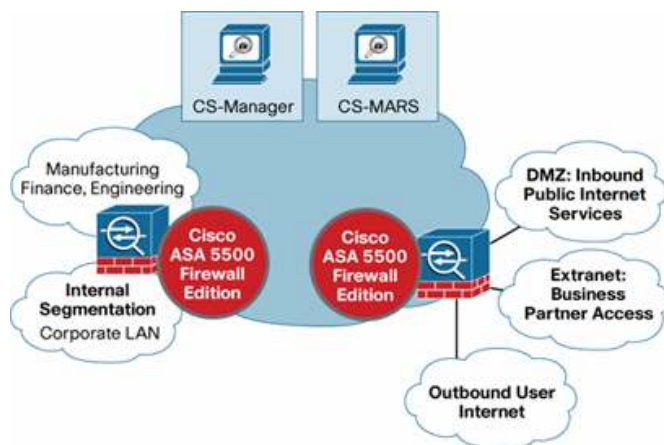
Figure 1. Solution Architecture
