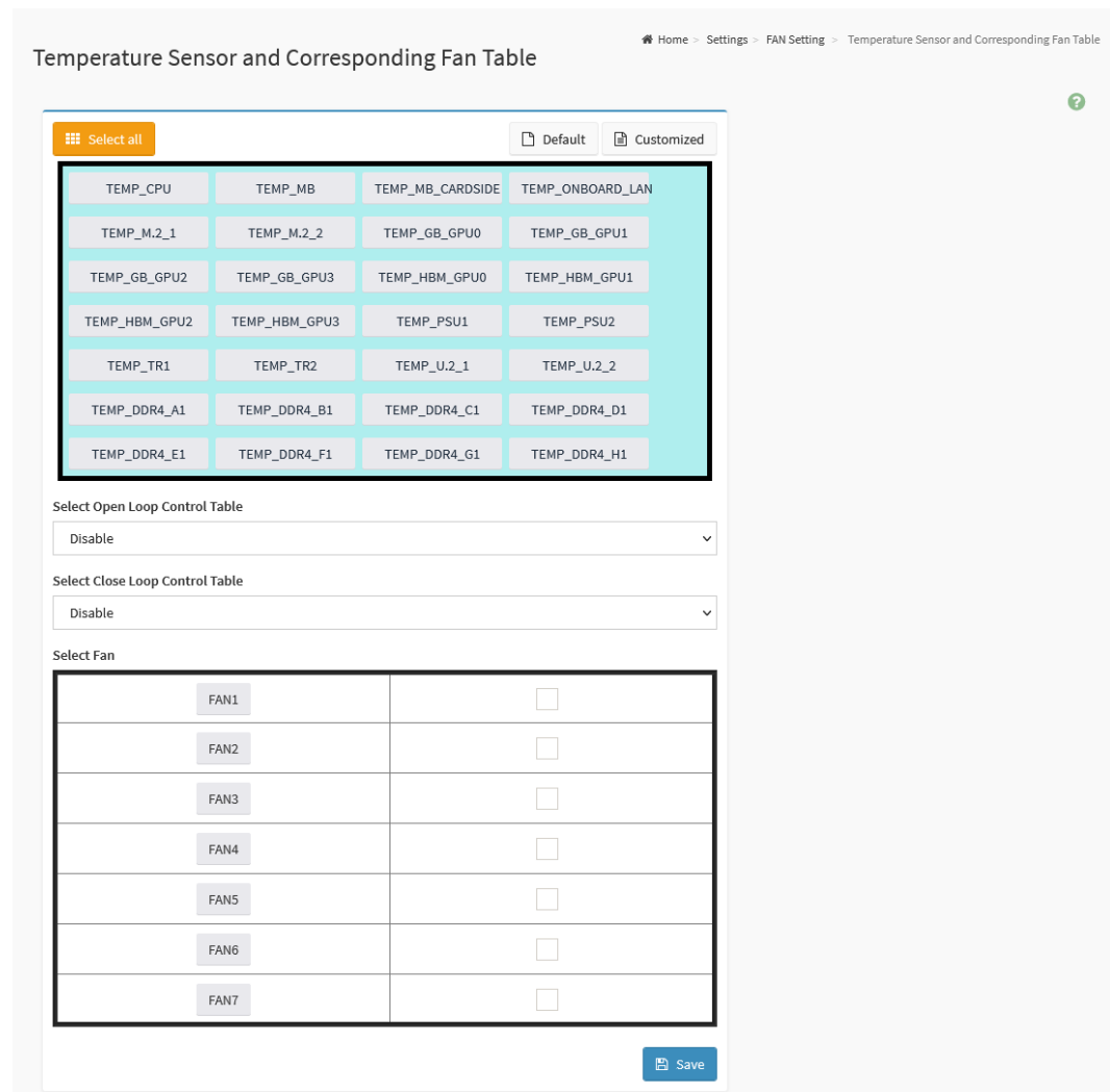
Figure 97. Snapshot of Temperature Sensor and Corresponding Fan Table Page
