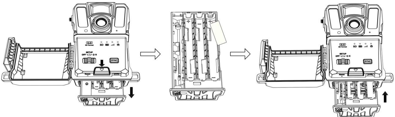
Figure 2-1 Install Batteries
