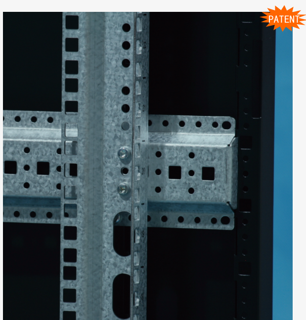
Fingerprint-resistant Zinc Mounting Profiles
