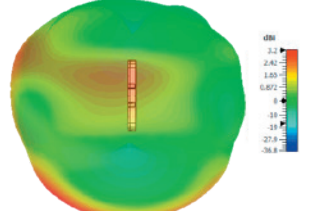
3D Plot Element D Top (2600 MHz)
