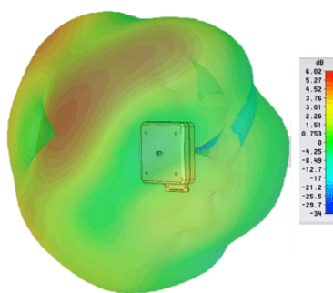
3D Gain Plot (2400MHz)
