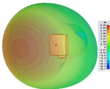
3D Gain Plot (850MHz)
