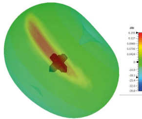
3D Pattern Element 2 (650MHz)
