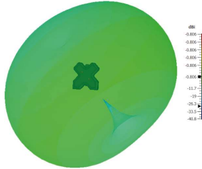
3D Pattern Element 3 (650MHz)
