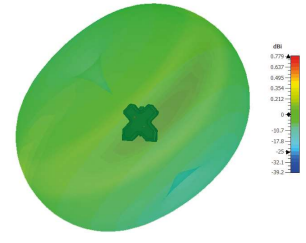
3D Pattern Element 4 (650MHz)
