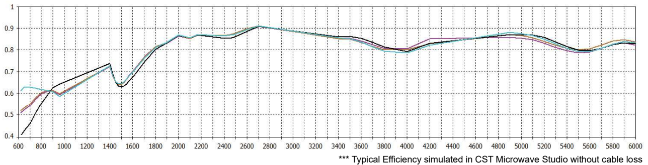
Typical Efficiency ***
